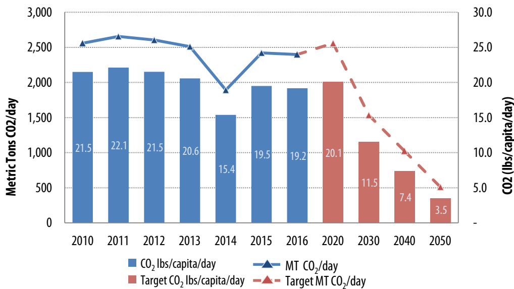
Figure 7.3 – Historic and Target Santa Cruz County Greenhouse Gas Emissions from Transportation
