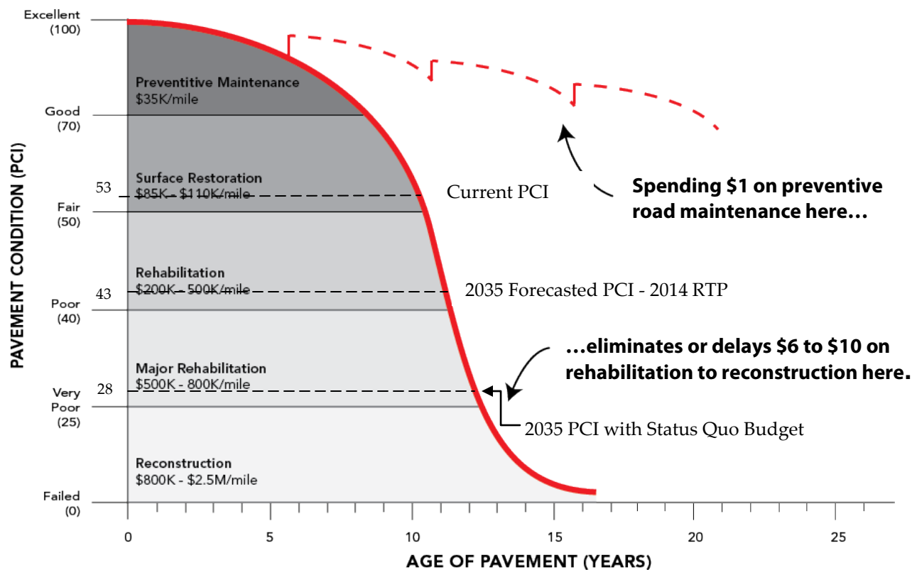
Figure D.34 – Pavement Deterioration Curve - Cost per Mile to Maintain Local Roads
