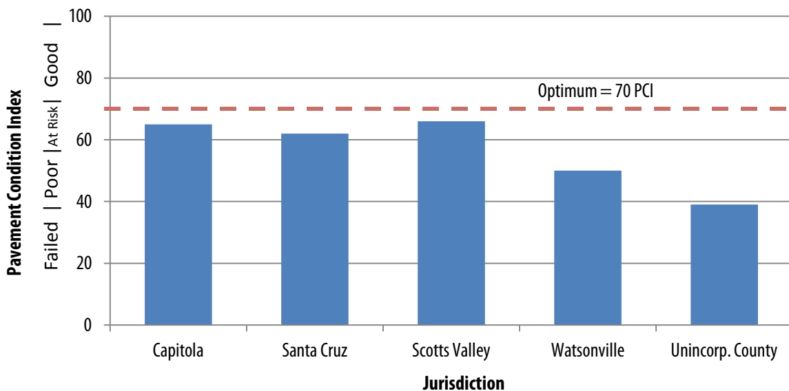
Figure 2.2 – Average Pavement Condition for Local Jurisdictions
